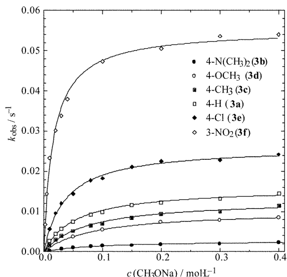
Figure 4. Observed rate constant of the cyclisation ( k_{\text{obs}}/\text{s}^{-1} ) of the 2-(benzoylamino)thiobenzamides 3a–f vs. the sodium methoxide concentration ( c/\text{mol}\cdot\text{L}^{-1} ) at 25 °C
