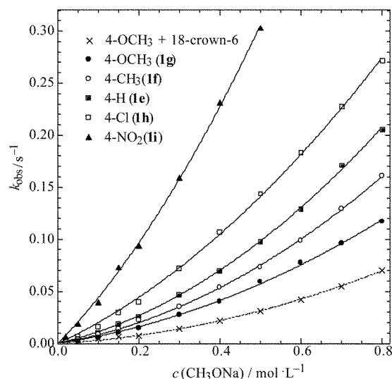
Figure 1. Observed rate constant of the cyclisation ( k_{\text{obs}}/\text{s}^{-1} ) of the 2-[(benzoyl)(methyl)amino]benzamides 1e–i vs. the concentration of sodium methoxide ( c/\text{mol}\cdot\text{L}^{-1} ) at 25 °C
