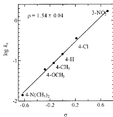
Figure 5. Hammett correlation of the cyclisation rate constant ( k_c ) of the 2-(benzoylamino)thiobenzamides 3a–f
