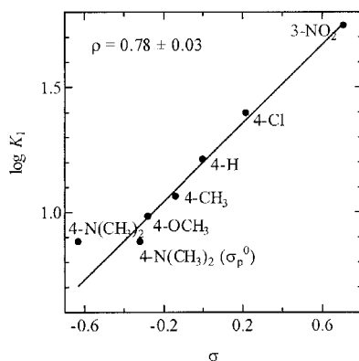
Figure 6. Hammett correlation of the equilibrium constant of the deprotonation ( K_1 ) of the 2-(benzoylamino)thiobenzamides 3a–f
