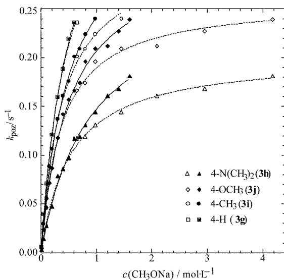
Figure 3. Observed rate constant of the cyclisation ( k_{\text{obs}}/\text{s}^{-1} ) of the 2-[(benzoyl)(methyl)amino]thiobenzamides 3g–j vs. the concentration c (solid symbols and solid lines) and vs. the apparent concentration c' (open symbols and dashed lines) of sodium methoxide ( c/\text{mol}\cdot\text{L}^{-1} ) calculated by means of the H_{\text{M}} function and Equation (5) at 25 °C
